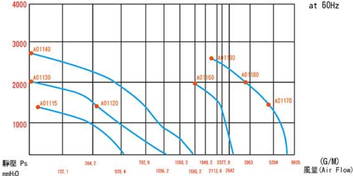
RB 型性能表 ( Characteristic curves )
